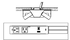
Double-Sided Conference Table Topmount (Both Sides)
