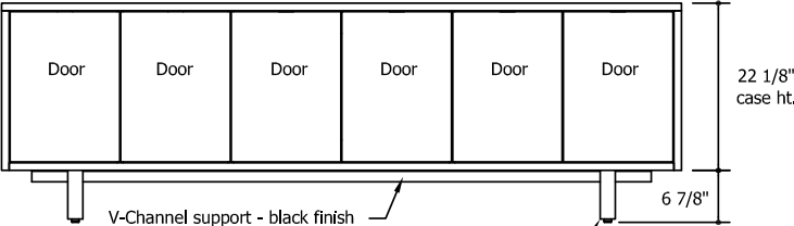
Conference Height Credenza
