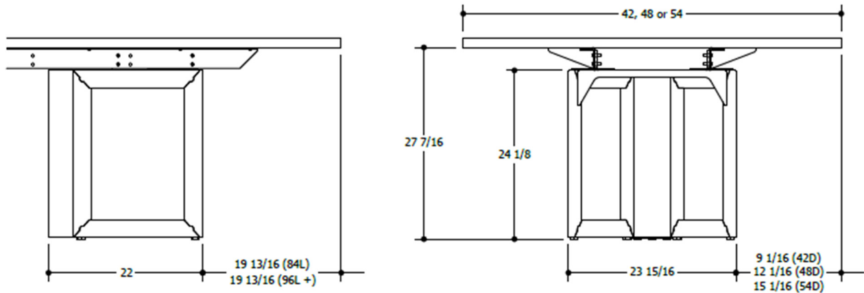
END BASE ELEVATION, 42, 48 & 54D
