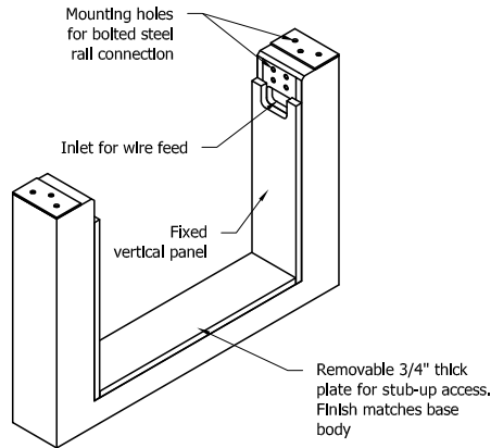
Large base : 72" Deep Tables "ON" Open Base, no metal trim
