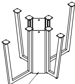
Removable Access panels - 9 3/4" diameter clear opening at floor for stub-up "XEP"- base
