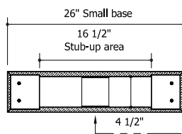
Horizontal section of Small Base
