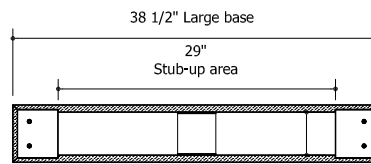
Horizontal section of Large base
