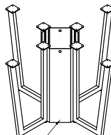
Removable Access panels - 9 3/4" diameter clear opening at floor for stub-up "XP"- base
