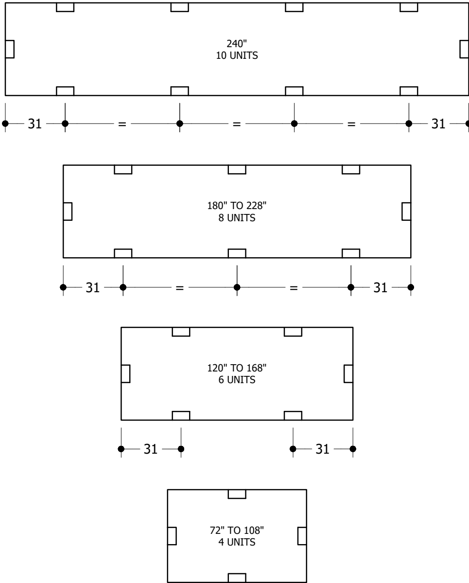
POWER LOCATIONS & QUANTITY BY TABLE LENGTH
