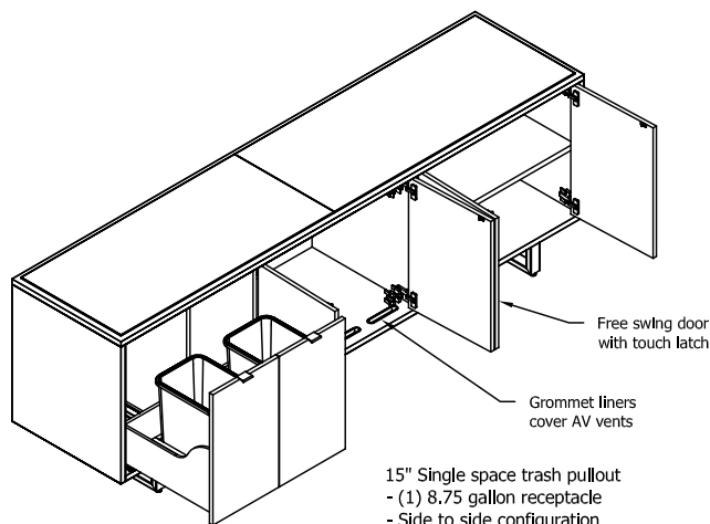
Front of Credenza
