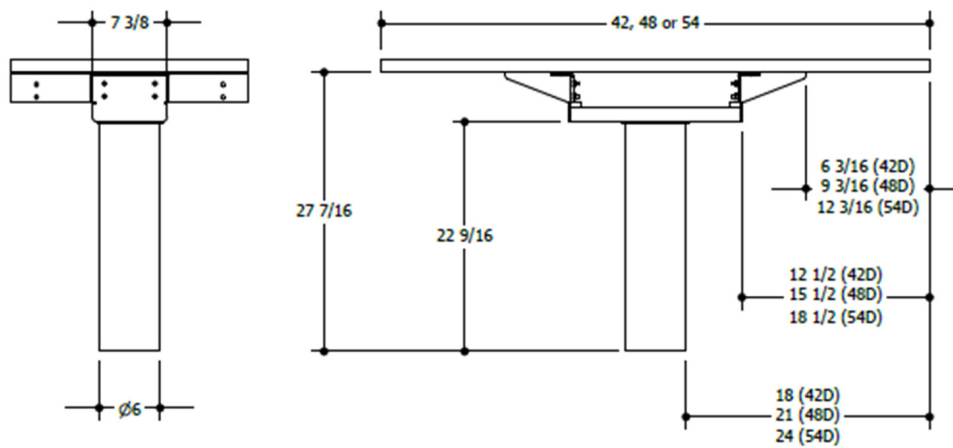
INTERMEDIATE COLUMN ELEVATIONS, 42, 48 & 54D
