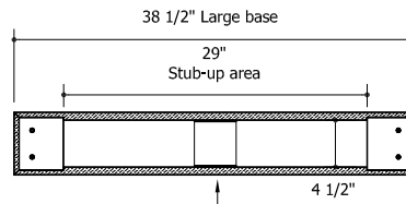
Horizontal section of Large base
