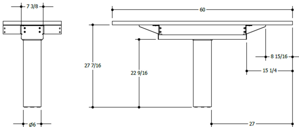
SIDE ELEVATION
