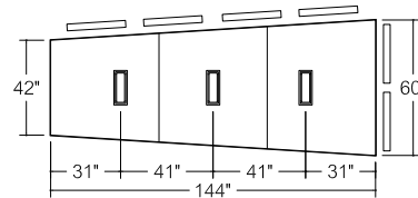
O2T60X144 11 Person Table
