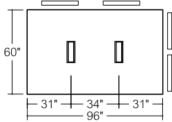
O2R60X96 8 Person Table
