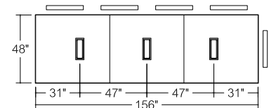
02R48X156 10 - 12 Person Table
