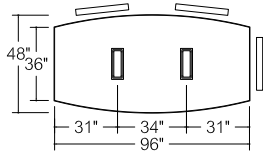
O2B48X96 6 Person Table
