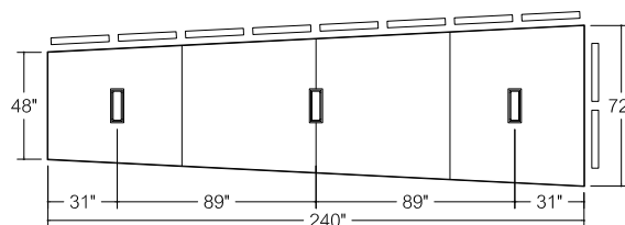
02T72X240 19 Person Table
