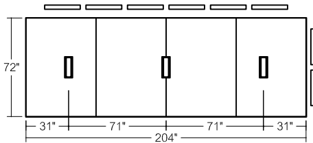
03R72X204 16 Person Table
