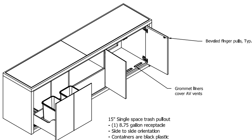
Front of Credenza
