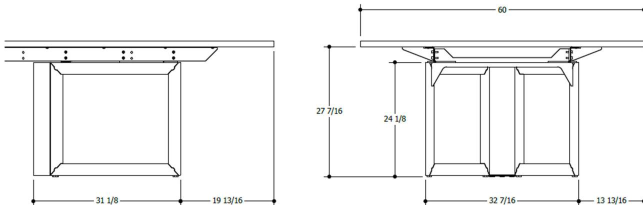
END BASE ELEVATION, 60D
