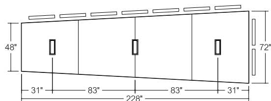
02T72X228 17 Person Table
